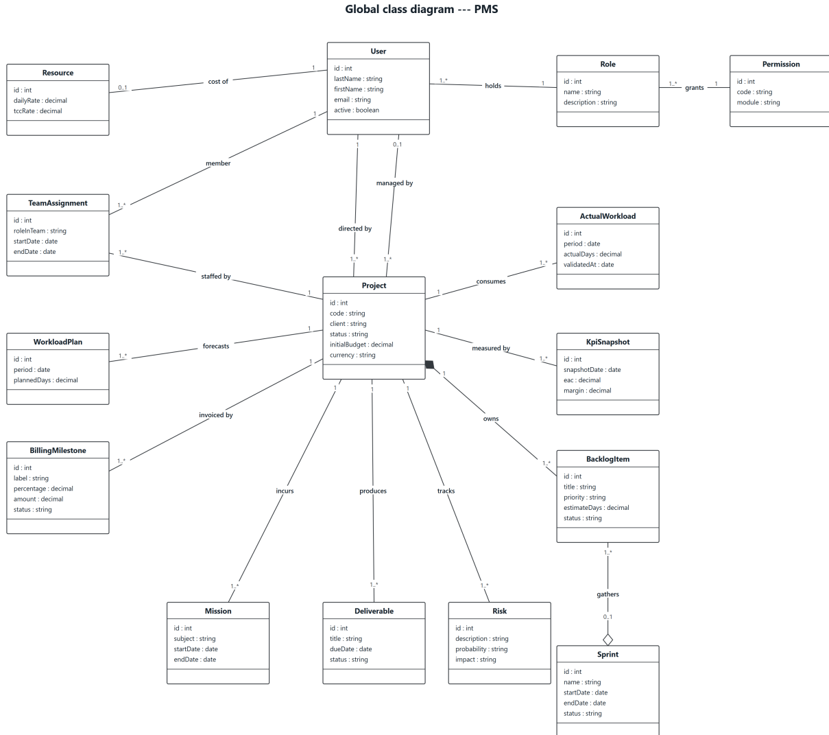
Figure 3.5: Domain model — principal classes and their associations
